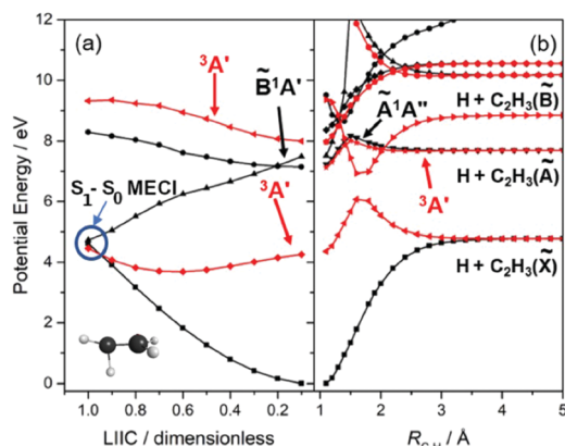
Fig. 2 Singlet (in black) and triplet (in red) PECs for C_2H_4 . Panel (a) is for a sequence of geometries along a LIIC connecting the optimised ground state geometry to that of the MECL linking the 1\pi\pi^* and S_0 PESs, the structure of which is shown. The curves shown in panel (b) are from a rigid body scan wherein R_{C-H} is extended at planar geometries, with the rest of the nuclear framework held at its ground state equilibrium geometry.
