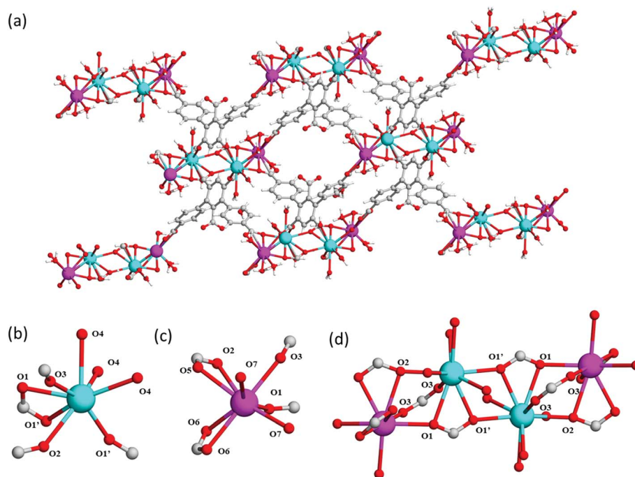
Fig. 4 View of (a) the crystal structure of MFM-512 along the a -axis; (b) type I) and (c) type II Ba(II) nodes in MFM-512 showing distorted octahedral and trigonal prismatic square face monocapped coordination, respectively. H-atoms are omitted for clarity; (d) View of the tetranuclear Ba(II) cluster in MFM-512. Carbon, grey; oxygen, red; hydrogen, white; barium, magenta (type I) and cyan (type II).
