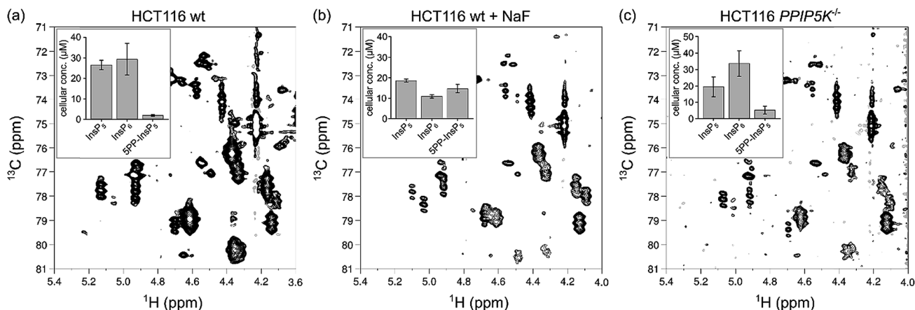
Fig. 6 Changes in 5PP-InsP 5 levels can be observed by NMR spectroscopy. (a) ^1\text{H} , ^{13}\text{C} HMQC spectrum of a HCT116 wt cell extract. (b) ^1\text{H} , ^{13}\text{C} HMQC spectrum of an extract of HCT116 wt cells treated with 10 mM NaF before extraction. (c) ^1\text{H} , ^{13}\text{C} HMQC spectrum of HCT116 PPIP5K -/- cell extract. The inserts display triplicates of absolute cellular concentration of InsP 5 , InsP 6 and 5PP-InsP 5 based on packed cell volume.
