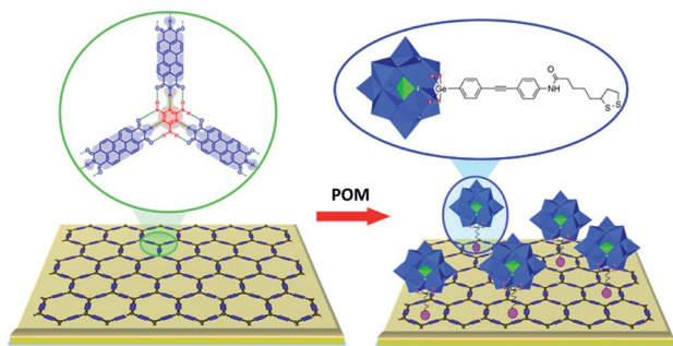
Fig. 13 Schematic depiction of the organisational preferences of the Keggin-type POM-based inorganic-organic hybrid units [PW_{11}O_{39}Ge(p-C_6H_4-C\equiv C-C_6H_4-NHC(O)(CH_2)_4(-CH-(CH_2)_2S-S-))_4]^{4-} (right) on the PTCDI/melamine-templated gold surface (left). Colour code: W, blue; P, green polyhedra; O, red spheres. Adapted with permission from ref. 29. Copyright 2016 American Chemical Society.
