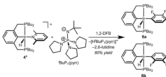
Scheme 4 C–H activation of 1,2-DFB by deprotonation of 4 + .
