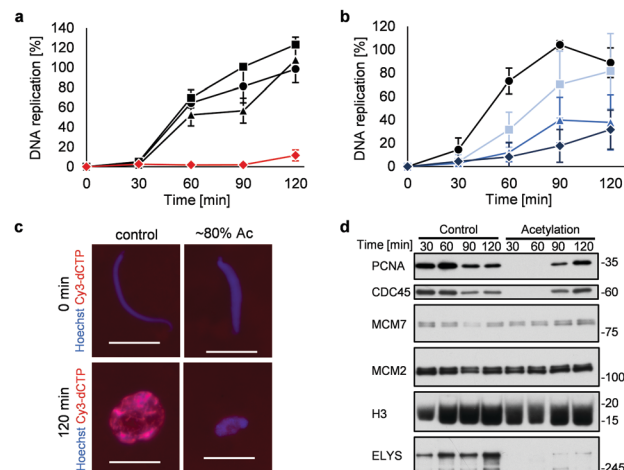
Fig. 4 Synthetic histone acetylation inhibits DNA replication. (a and b) XSC (20 000 sperm per \mu\text{L} ) was treated with 2 (30 \mu\text{M} ) and 6 (30 mM) for (a) 7 h or (b) the indicated time at 25 ^{\circ}\text{C} . After the reaction, control or acetylated XSC was incubated with interphase egg extracts containing radiolabeled [ \alpha - ^{32}\text{P} ]-dCTP. The DNA replication kinetics in egg extracts was assessed by the incorporation of radioactivity, determined using a scintillation counter. Data shown are the average and SD (bars) from (a) three or (b) five independent experiments. (a) ●: control; ■: 2 only; ▲: 6 only; ◆: 2 + 6 . (b) ●: control. Reaction time = ■: 0.5 h; ▲: 1 h; ◆: 3 h. (c) and (d) XSC (20 000 sperm per \mu\text{L} ) was treated with 2 (30 \mu\text{M} ) and 6 (30 mM) for 7 h. (c) Control or acetylated XSC was incubated with interphase egg extracts containing Cy3-dCTP. After incubation, the samples were fixed and DNA was visualized with Hoechst 33258 (blue image). DNA replication was monitored as the incorporation of Cy3-dCTP (red image) into DNA. The scale bar represents 20 \mu\text{m} . (d) Control or acetylated XSC was incubated with interphase egg extracts. Chromatin was isolated from the egg extracts at the indicated times and the chromatin samples were analyzed by immunoblotting using the indicated antibodies.
