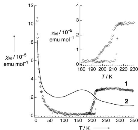
Fig. 6 Temperature dependence of magnetic susceptibility ( \chi_M ) of \text{Pt}_2(\text{EtCS}_2)_4\text{I} (2) and \text{Pt}_2(n\text{-BuCS}_2)_4\text{I} (1; O: 1st cooling, +: 1st heating, Δ: 2nd cooling). Inset shows the phase transition behavior at around 210 K of 1. Adapted with permission from ref. 33. Copyright 2002 Wiley-VCH.
