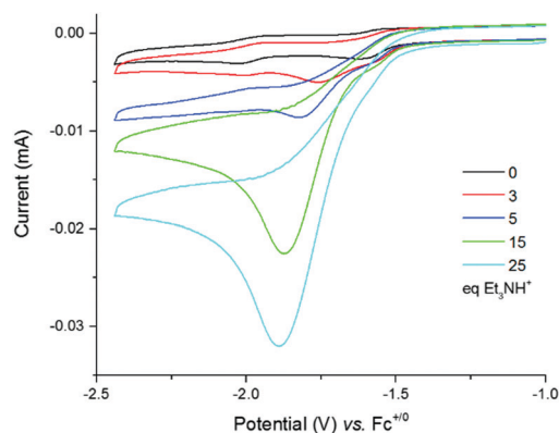
Fig. 3 Cyclic voltammograms of a 0.25 mM solution of 4 in DMF (0.1 M NEt 4 ClO 4 ) with increasing amounts of Et 3 NHCl (0–25 equiv.) recorded at a glassy carbon electrode (3 mm diameter) and 100 mV s -1 .
