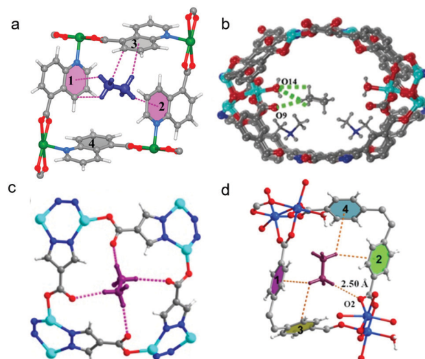
Fig. 13 Preferential ethane binding sites in \text{C}_2\text{H}_6/\text{C}_2\text{H}_4 selective adsorbents: (a) Qc-5-Cu-sql- \beta as determined by NPD experiments; 109 (b) TJT-100, as determined by GCMC simulations; 70 (c) JNU-2, as determined by DFT-D calculations; 121 (d) NUM-7a, as determined by GCMC simulations. 117 (Reprinted with permissions from ref. 109, 70, 121 and 117; copyright 2018, American Chemical Society; copyright 2018, Wiley-VCH Verlag GmbH & Co. KGaA, Weinheim; copyright 2019, American Chemical Society; copyright 2020, American Chemical Society.)
