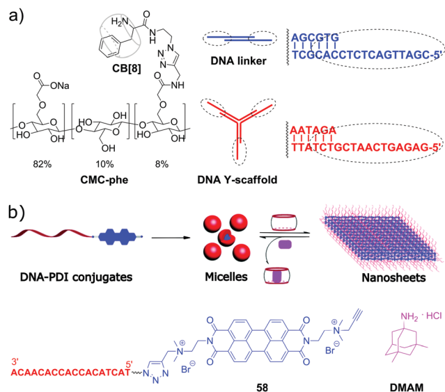
Scheme 12 (a) Molecular building blocks self-assembling into a double network hydrogel based on the interpenetrating CB[8]- and DNA-based networks; (b) structure of the ssDNA-perylenediimide (PDI) conjugates, schematic representation of their self-assembly into spherical micelles and rearrangement into nanosheets upon addition of CB[10]. Adapted from ref. 95, copyright RSC.
