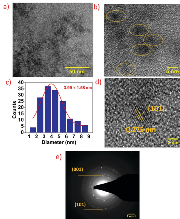
Fig. 2 (a and b) TEM image of the synthesized SnS 2 QDs, (c) size distribution of SnS 2 QDs, calculated average diameter of SnS 2 QDs is 3.99 \pm 1.58 nm, (d) HRTEM lattice fringes of SnS 2 QDs, and (e) SAED pattern of SnS 2 QDs.
