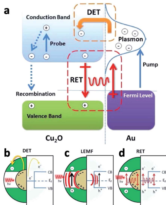
Fig. 14 Various possible energy-transfer and separation processes responsible for plasmon-enhanced photocatalytic activity of \text{Cu}_2\text{O} /Au-based HNS. 125 (a) Scheme of energy absorption at the metal (pump) and the subsequent energy-transfer processes: (b–d) illustration of the metal core (Au) and the SC shell ( \text{Cu}_2\text{O} ) energy positions (right) and processes (left): (b) direct energy transfer (DET), where LSPR 'hot' electrons are transferred to the SC's CB; (c) local electromagnetic field enhancement (LEMF), where the e^- – h^+ charge-separation in the SC is radiatively aided by the metal excitation; (d) resonant energy transfer (RET), where the LSPR dipole induces e^- – h^+ pair separation in the SC via a non-radiative mechanism that relaxes the localized surface plasmon dipole. Adapted with permission from the American Chemical Society, copyright 2012.
