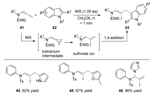
Scheme 14 NIS-mediated intermolecular iodofunctionalization of allenamides with indoles, pyrrole, and furan.
