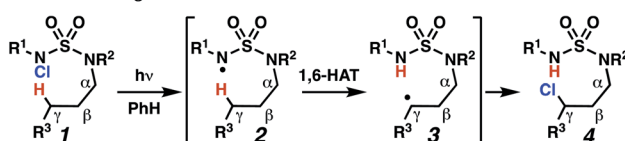
Scheme 1 \gamma -C(sp 3 )–H reactions of amine derivatives.
