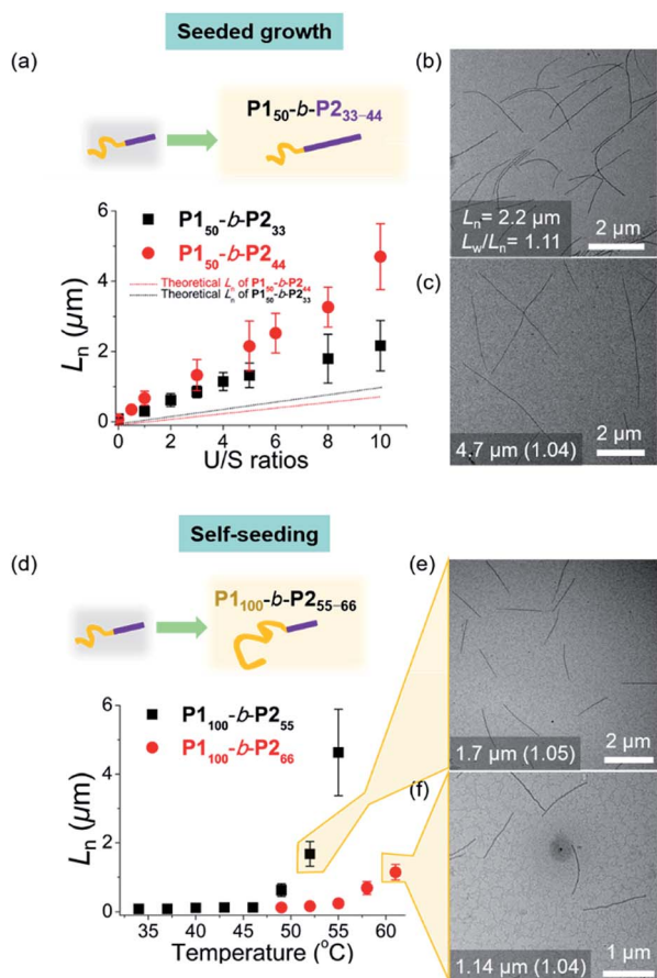
Fig. 6 Living CDSA for larger BCPs. For P1 50 - b-P2 33–44 , (a) plots of U/S ratios versus L_n showing successful seeded growth, and the solid lines represented theoretical L_n values. TEM images of U/S ratios = 10 for (b) P1 50 - b-P2 33 , and (c) P1 50 - b-P2 44 . For P1 100 - b-P2 55–66 , (d) plots of annealing temperature (°C) versus L_n showing CDSA through self-seeding. TEM images of the micron-sized 1D nanofibers from (e) P1 100 - b-P2 55 , and (f) P1 100 - b-P2 66 via self-seeding. The number in images indicates "the average L_n and its length dispersity".
