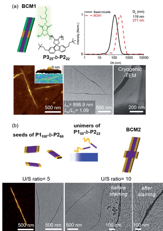
Fig. 7 More complex BCMS were prepared by (a) adding a unimer P3 25 -b-P2 22 having a different block to P1 50 -b-P2 22 seed (BCM1) and (b) adding a unimer ( P1 50 -b-P2 22 ) to a wider seed ( P1 100 -b-P2 66 ) to produce BCM2 with different widths. The number in an image (a) indicates "the average L_n and its length dispersity".
