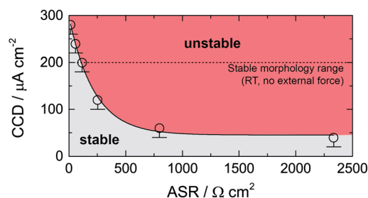
Fig. 3 Critical current density (CCD) as a function of the area specific resistance (ASR). Solid line represents an exponential function. The dashed line indicates the theoretical limit as suggested by theoretical considerations using a relaxation model. 31 See text for further explanation.
