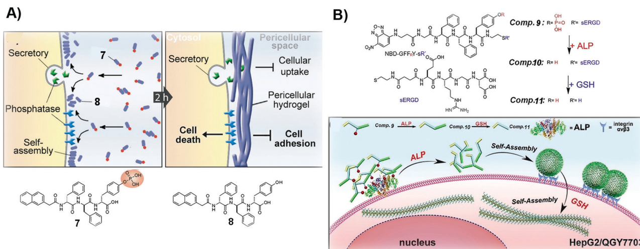
Fig. 2 (A) Illustration of the formation of a pericellular hydrogel and the molecular structures of 7 and 8 . (B) Molecular structures of 9 – 11 and the diagram of the process of tandem self-assembly. Reproduced with permission from ref. 39 and 46.
