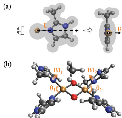
Fig. 2 (a) An illustration of Sterimol parameters for imidazole N-donor substituted with \text{CH}_3 , where L is length of the group along a user-defined axis ( \text{Cu}-\text{N} ) and B1 is the minimum width when looking down from the axis. The third Sterimol parameter, which is the corresponding maximum width, B5 , is not shown here. (b) Representation of strain descriptors \theta and B1 in TS oxo . All strain descriptors are calculated using optimized IS geometries. (Cu: ochre, O: red, N: blue, C: grey).
