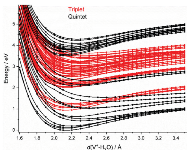
Fig. 2 Splined potential energy surface scans for the relevant quintet and triplet states along the water dissociation coordinate d(\text{V}^+-(\text{H}_2\text{O})) on the CASSCF(4,9)/aug-cc-pVDZ level of theory, respectively. All other internal coordinates are kept at the values calculated for the minimum.
