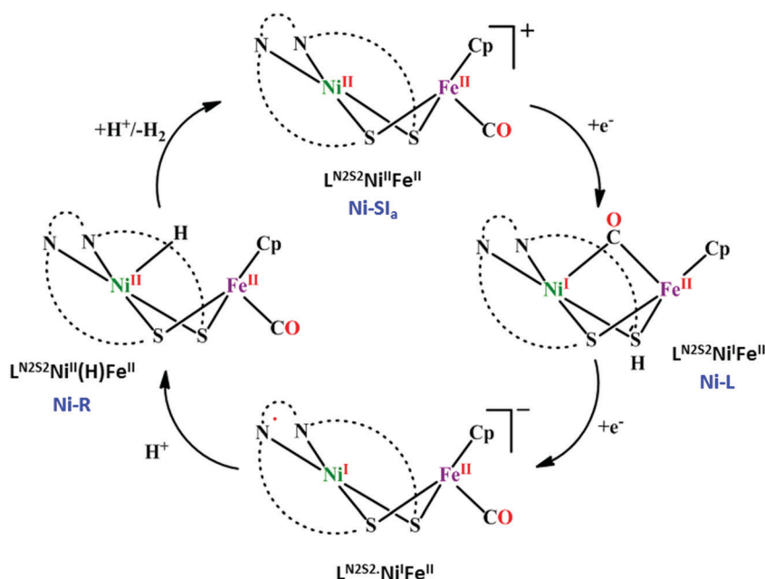
Scheme 32 Proposed mechanistic cycle of proton reduction in complex [\text{L}^{\text{N2S2}}\text{Ni}^{\text{II}}\text{Fe}^{\text{II}}\text{cp}(\text{CO})]^+ (Fig. 32b).
