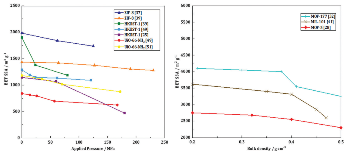
Fig. 3 BET SSA as a function of applied pressure during pelletization (left): (▲) – ZIF-8 by Ribeiro et al. , 37 (▲) – ZIF-8 by Bazer-Buchi et al. , 39 (●) – UiO-66-NH 2 by Peterson et al. , 51 (●) – UiO-66-NH 2 by Dhainaut et al. , 49 (■) – HKUST-1 by Bazer-Buchi et al. , 39 (■) – HKUST-1 by Dhainaut et al. , 49 and (■) – HKUST-1 by Alcañiz-Monge et al. , 25 BET surface area as a function of bulk density (right): (+) – MOF-177 by Zacharia et al. , 32 (x) – MIL-101 by Ardelean et al. , 41 and (♦) – MOF-5 by Purewall et al. 28
