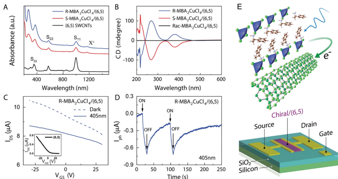
Fig. 13 (A) UV-Vis-NIR absorption spectra of SWCNT, R- and S-MBA 2 CuCl 4 /SWCNT. (B) CD signals of R- and S-MBA 2 CuCl 4 /(6,5) SWCNT and (rac-MBA) 2 CuCl 4 /(6,5) SWCNT. (C) A comparison of the effects of dark and photoresponse conditions on the FET transfer curve. (D) The photocurrent response of (R\text{-MBA})_2\text{CuCl}_4/\text{SWCNT} over time. (E) A schematic description of a three-terminal FET device. Reprinted with permission. 104 Copyright 2021, American Chemical Society.
