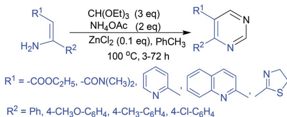
Scheme 1 Synthesis of 4,5-disubstituted pyrimidine analogs via ZnCl_2 -catalyzed three-component coupling reaction.
