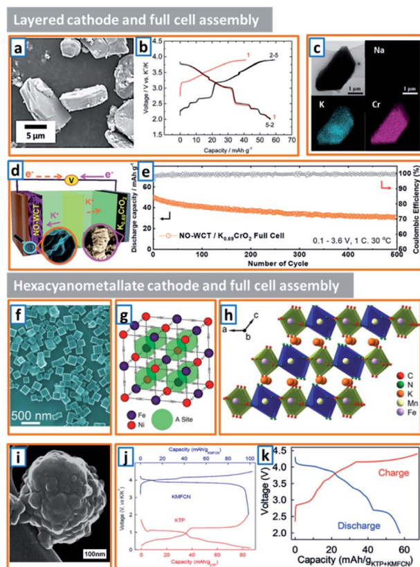
Fig. 22 Full cell assembly with counterpart cathodes (layered cathodes and hexacyanometallate cathodes). (a) SEM images of P2\text{-K}_{0.41}\text{CoO}_2 and (b) charge and discharge curves of \text{K}/P2\text{-K}_{0.41}\text{CoO}_2 cell. Reproduced with permission. 158 Copyright 2017, The Royal Society of Chemistry. (c) TEM images and the corresponding EDX mapping of P3\text{-K}_x\text{CrO}_2 . Reproduced with permission. 159 Copyright 2018, The Royal Society of Chemistry. (d) Schematic illustration of a K-ion full cell using a NO-WCT anode and P3\text{-K}_{0.69}\text{CrO}_2 cathode, and (e) the corresponding deep cycling performance. Reproduced with permission. 19 Copyright 2019, The Royal Society of Chemistry. (f) SEM image of potassium iron hexacyanoferrate dihydrate particles. Reproduced with permission. 161 Copyright 2016, Wiley. (g) Face-centered cubic structure of NiHCF with Prussian blue crystal structure. Reproduced with permission. 162 Copyright 2011, American Chemical Society. (h) Structural illustration and (i) morphology of KMHCF powder. Reproduced with permission. 163 Copyright 2017, American Chemical Society. (j) Voltage profiles of KMFCN cathode and KTP@C anode, and (k) the corresponding charge/discharge curve of potassium full cell. Reproduced with permission. 35 Copyright 2019, Wiley.
