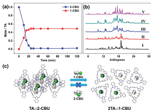
Fig. 4 (a) Time-dependent solid-vapor sorption plot of TA \supset 2-CBU after exposure to 1-CBU vapor. (b) Time-dependent PXRD pattern of (I) initial TA \supset 2-CBU ; TA \supset 2-CBU after adsorption of 1-CBU vapor for (II) 10 minutes; (III) 20 minutes and (IV) 30 minutes; (V) simulated pattern produced from the single crystal structural data for 2TA \supset 1-CBU . (c) Illustration showing the reversible and irreversible structural transformation between TA \supset 2-CBU and 2TA \supset 1-CBU .
