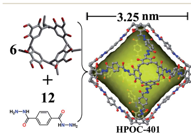
Fig. 3 Schematic illustration of the assembly of the [6 + 12] octahedron based on C4RACHO and the linear terephthalohydrazide linker and its X-ray crystal structure. The hydrogen atoms and iso -butyl groups are omitted for clarity.
