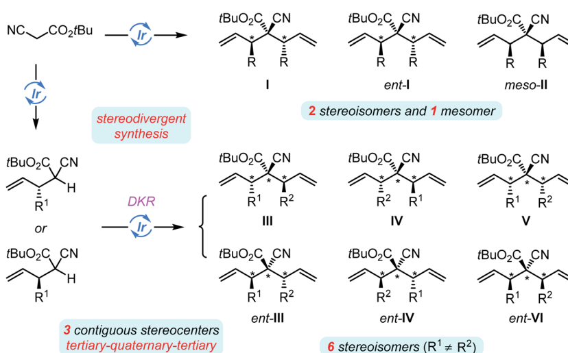
Scheme 2 Ir-catalyzed double-asymmetric allylic alkylation ((a) previous work) and stereodivergent double allylation ((b) this work).
