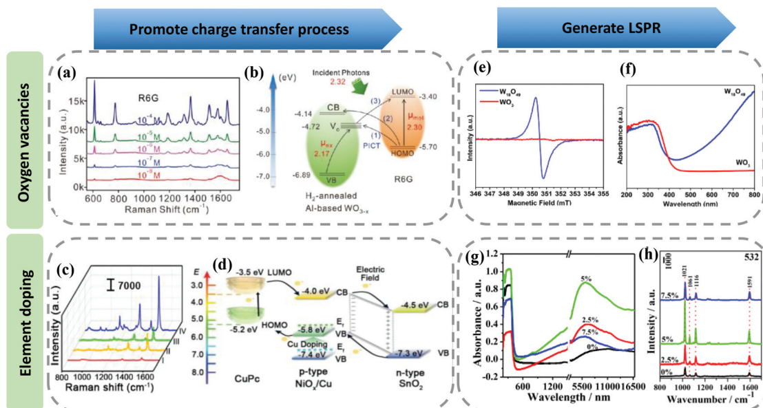
Fig. 9 (a) SERS spectra of R6G molecules adsorbed on \text{WO}_{3-x} substrate at different concentrations. (b) Schematic showing the energy level diagram of R6G on \text{WO}_{3-x} and the charge transfer process in this system. Reproduced with permission from ref. 103 (Copyright © 2019 WILEY-VCH Verlag GmbH & Co. KGaA, Weinheim). (c) SERS spectra of copper phthalocyanine (CuPc) molecules on Si(I), \text{SnO}_2 (II), \text{SnO}_2 -NiO (III), and Cu-doped \text{SnO}_2 -NiO (IV) substrates. (d) Schematic presenting the energy level diagram of CuPc on Cu-doped \text{SnO}_2 -NiO and the charge transfer process. Reproduced with permission from ref. 105 (Copyright © 2021 Wiley-VCH GmbH). (e) Electron paramagnetic resonance (EPR) spectra of the \text{W}_{18}\text{O}_{49} and \text{WO}_3 mesocrystals. (f) UV-vis spectra of \text{W}_{18}\text{O}_{49} and \text{WO}_3 mesocrystals. Reproduced with permission from ref. 25 (Copyright © 2021, American Chemical Society). (g) FTIR absorption spectra of Ga-doped ZnO nanoparticles combined with the UV-vis-NIR absorption spectra. (h) SERS spectra of MPy on Ga-doped ZnO substrate with different doping ratios. Reproduced with permission from ref. 107 (Copyright © 2021, American Chemical Society).
