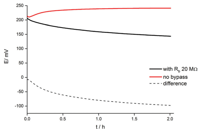
Fig. 6 Dependence of open circuit potential on time for a potassium-selective ISE, non-bypassed (red line) and bypassed (black line) by zinc wire and resistor R_b = 20\text{ M}\Omega . Dashed line: difference of potentials in the presence and absence of bypass.
