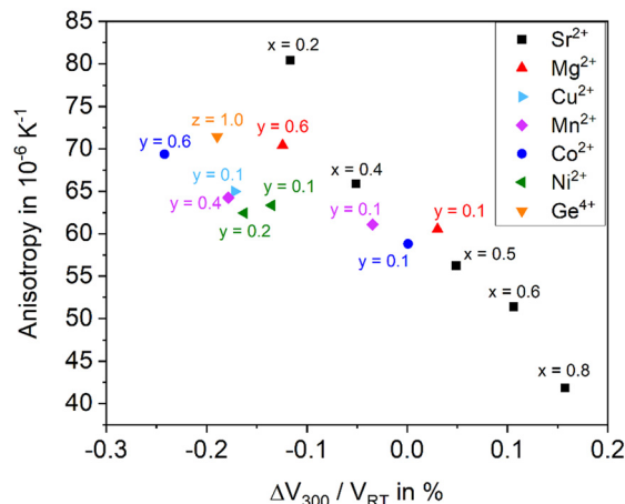
Fig. 13 Anisotropy versus the mean change of the volume of \text{Ba}_{1-x}\text{Sr}_x\text{Zn}_{2-y}\text{M}_y\text{Si}_{2-z}\text{Ge}_z\text{O}_7 samples. If the \text{Sr}^{2+} concentration varies on the expense of \text{Ba}^{2+} , \text{Zn}^{2+} is not substituted ( y = 0 , i.e., sample series \text{Ba}_{1-x}\text{Sr}_x\text{Zn}_2\text{Si}_2\text{O}_7 ). If \text{Zn}^{2+} or \text{Si}^{4+} are replaced, the x -value is kept constant with x = 0.5 (sample series \text{Ba}_{0.5}\text{Sr}_{0.5}\text{Zn}_{2-y}\text{M}_y\text{Si}_{2-z}\text{Ge}_z\text{O}_7 ).
