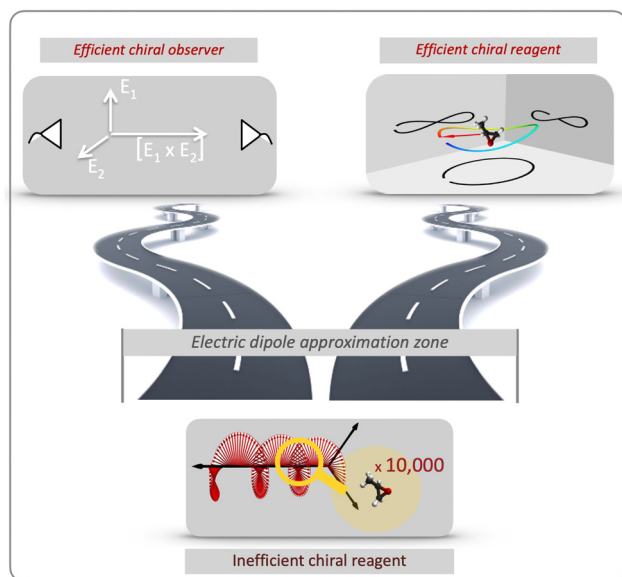
Fig. 2 Two roads to efficient enantio-discrimination: chiral reagent (approaches that substitute the inefficient (non-local) light helix in space by an efficient (local) light helix in time) and chiral observer (approaches that do not rely on the chiral properties of light).
