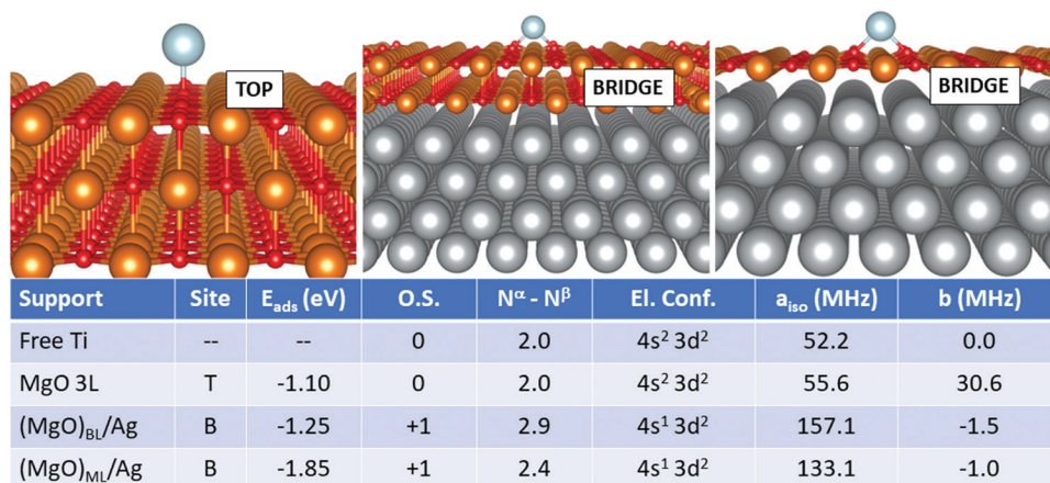
Fig. 1 Ti adatom. Most favourable adsorption mode on MgO 3L (left), (MgO) BL /Ag (middle) and (MgO) ML /Ag (right). Adsorption site (T = O top, B = bridge), adsorption energy ( E_{\text{ads}} ), formal oxidation state of the adatom (O.S.), number of unpaired electrons ( N^{\alpha}-N^{\beta} ), electron configuration (El. Conf.), and isotropic ( a_{\text{iso}} ) and anisotropic ( b ) hyperfine parameters.
