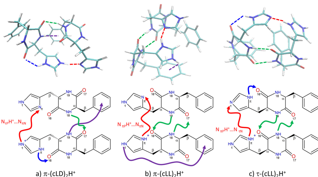
Fig. 2 Protonated dimers accounting for the experimental spectrum, calculated at the ri-b97-d-D3BJ/defT-TZVPPD level of theory. (a) \pi\text{-(c-LD)}_2\text{H}^+ , (b) \pi\text{-(c-LL)}_2\text{H}^+ , and (c) \tau\text{-(c-LL)}_2\text{H}^+ . Hydrogen bonds are indicated by dashed lines in the 3D structures (top) and by arrows in the 2D schemes (bottom). The strong ionic \text{NH}^+\cdots\text{N} interaction is shown in red, the neutral \text{NH}\cdots\text{O} interactions in green, the \text{NH}\cdots\pi interactions in purple, and the intramolecular \text{NH}\cdots\text{O} interaction in blue.
