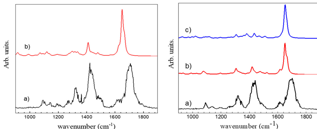
Fig. 3 Left: (a) Experimental IRMPD spectrum of \pi\text{-(c-LD)}_2\text{H}^+ in the fingerprint region. (b) Simulated spectrum for \pi\text{-(c-LD)}_2\text{H}^+ . Right: (a) Experimental IRMPD spectrum of \pi\text{-(c-LL)}_2\text{H}^+ in the fingerprint region. (b) Simulated spectrum for \pi\text{-(c-LL)}_2\text{H}^+ . (c) Simulated spectrum for \tau\text{-(c-LL)}_2\text{H}^+ .
