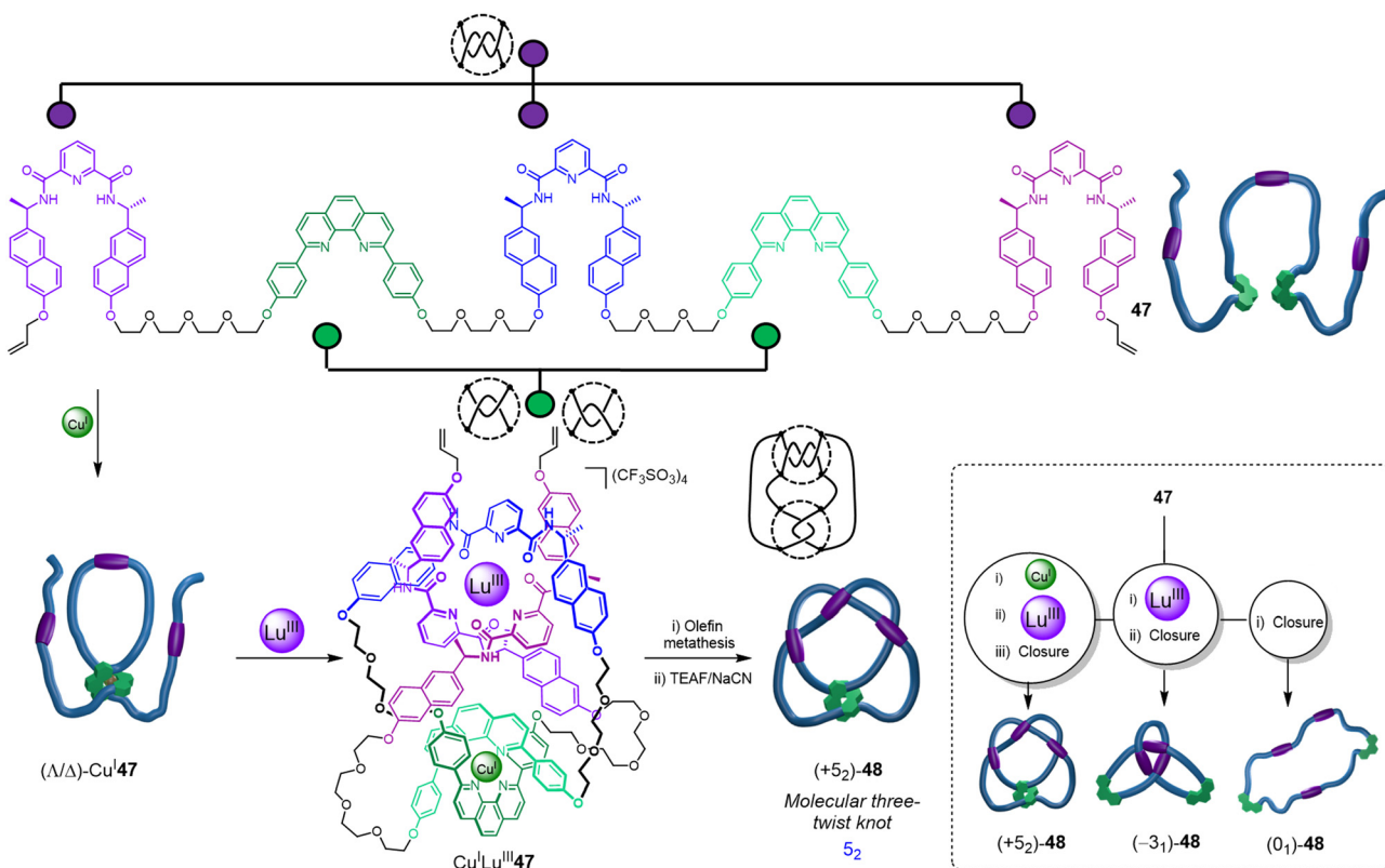
Fig. 16 Synthesis of a molecular 5_2 three-twist knot via stepwise folding around \text{Cu}^{\text{I}} and \text{Lu}^{\text{III}} templates, followed by covalent capture and demetallation. Tangles are shown next to crossing regions. Inset: A single ligand 47 forms three topoisomers: 5_2 knot (+5_2)\text{-48} , trefoil knot (-3_1)\text{-48} and unknot (0_1)\text{-48} . 21
