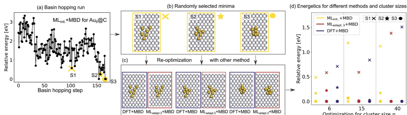
Fig. 4 (a) Basin hopping run with \text{ML}_{\text{init}} for \text{Au}_6@\text{C} with \text{Au}_6 nanoclusters (NCs). Yellow circles indicate (b) 3 selected structures S1–S3 that include the energetically lowest geometry and two randomly selected structures according to \text{ML}_{\text{init}} , that are (c) reoptimized with DFT+MBD (blue) and \text{ML}_{\text{adapt.3}} +MBD (red). (d) Relative energies reported with respect to the energetically lowest cluster for each method. In addition, energy rankings of the energetically lowest structures and two randomly selected structures from basin hopping runs with NC sizes of 15 and 40 atoms using \text{ML}_{\text{init}} +MBD (yellow), \text{ML}_{\text{adapt.3}} +MBD (red), and DFT+MBD (blue). Corresponding structures are shown for each method in Fig. S2.†
