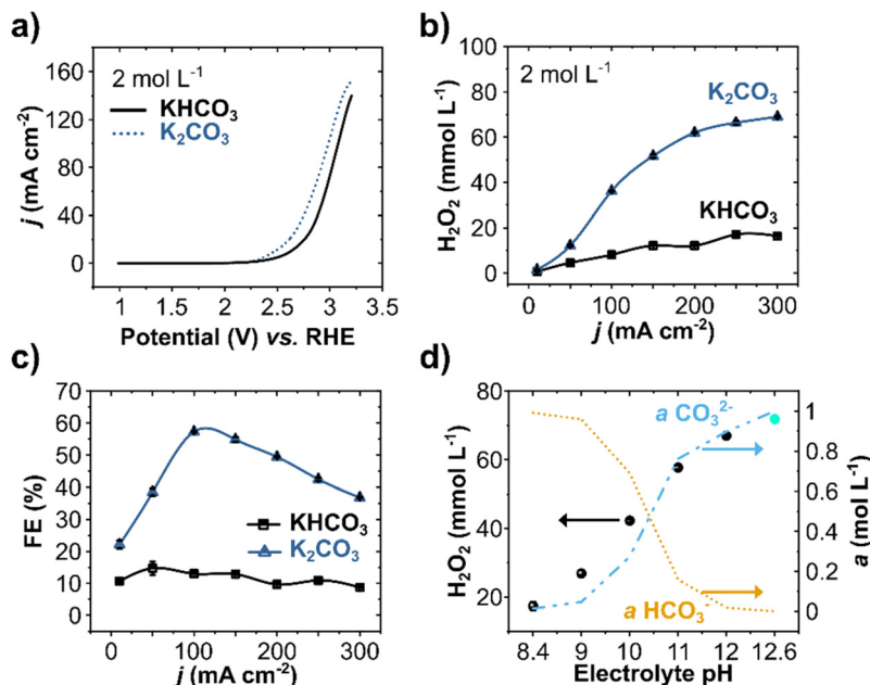
Fig. 1 WOR to \text{H}_2\text{O}_2 in 2 \text{ mol L}^{-1} \text{KHCO}_3 and \text{K}_2\text{CO}_3 electrolytes. (a) Anodic LSV starting from +0.18 V vs. Ag/AgCl (calculated vs. RHE) with a scan rate of 100 \text{ mV s}^{-1} . (b) \text{H}_2\text{O}_2 concentration and (c) FE at the indicated applied current densities for 10 minutes at each step. (d) Galvanostatic polarization at 300 \text{ mA cm}^{-2} for 10 minutes in 2 \text{ mol L}^{-1} \text{KHCO}_3 (at adjusted pH values from 8.4 to 12) and 2 \text{ mol L}^{-1} \text{K}_2\text{CO}_3 (pH 12.6) and the corresponding calculated ionic activity for \text{HCO}_3^- and \text{CO}_3^{2-} ions. The experiments were performed using a 5 \text{ cm}^2 BDD anode in a two-compartment H-cell cooled in an ice bath. The electrolyte was changed between the galvanostatic steps and kept under constant stirring of 1000 rpm.
