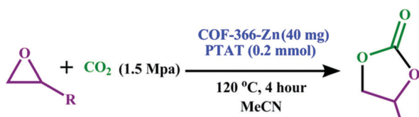
Scheme 7 The synthesis of cyclic carbonates via \text{CO}_2 incorporation using COF-366-Zn. Reproduced with permission from ref. 23; copyright: 2017, Dalton Transactions.
