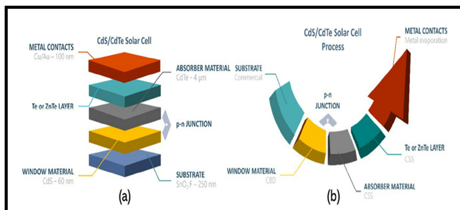
Fig. 18 CdS/CdTe solar cell device with architecture of (a) glass/FTO/CdS/CdTe/ZnTe/Cu/Au and (b) pictorial illustration of the junction development mechanism. Reprinted with permission from ref. 219. Copyright (2021), AIP Publications.
