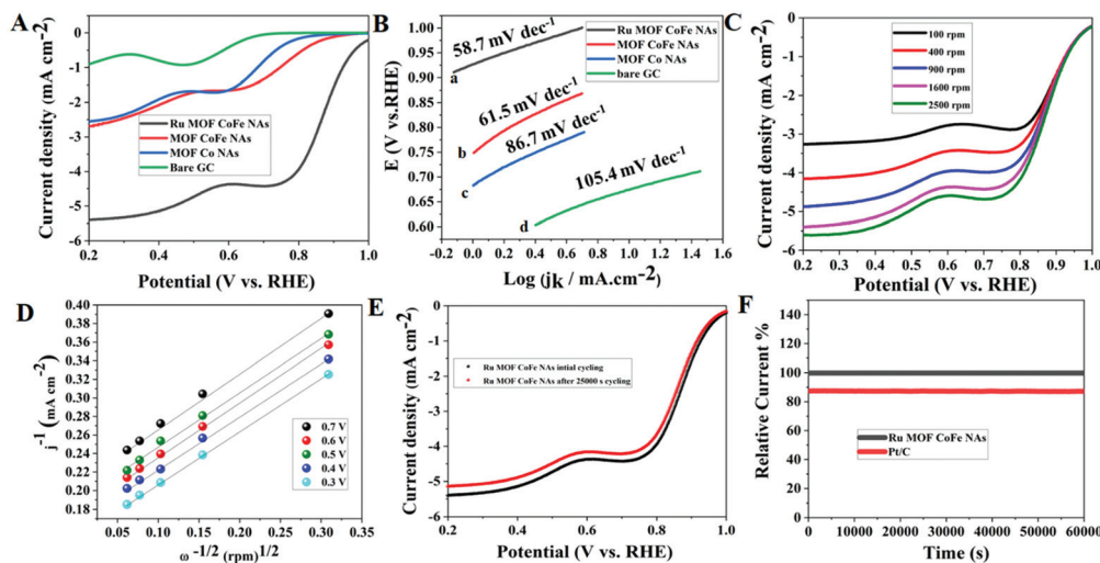
Fig. 5 (A) LSV curves of the various catalysts in \text{O}_2 -saturated 0.1 M KOH solution. (B) Corresponding Tafel plots for various catalysts. (C) LSV curves of the Ru MOF CoFe nanoarray catalyst in \text{O}_2 -saturated 0.1 M KOH solution at different rotation rates. (D) K–L plots measured at various potential values from 0.3 to 0.7 V vs. RHE. (E) Polarization curves of Ru MOF CoFe nanoarray catalyst before and after 25 000 s. (F) Long-term stability studies of Ru MOF CoFe nanoarrays and Pt/C catalyst in \text{O}_2 -saturated 0.1 M KOH.
