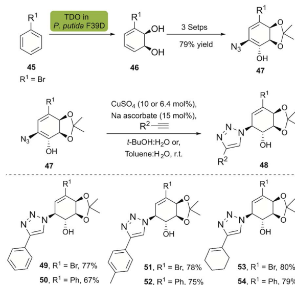
Scheme 5 Chemo-enzymatic synthesis of the bromoazidoconduritols derivative, and synthesis of triazolyconduritols.
