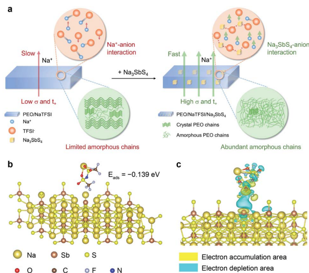
Fig. 1 Design of the interaction between the anion in salt and the additive. (a) Schematic illustrations of the PEO/ \text{NaTFSI} and PEO/ \text{NaTFSI} / \text{Na}_3\text{SbS}_4 electrolytes where the interactions between \text{Na}_3\text{SbS}_4 and \text{TFSI}^- anions are highlighted by red dotted lines. (b) The optimized configuration, adsorption energy, and (c) differential charge density of \text{NaTFSI} adsorbed on \text{Na}_3\text{SbS}_4 ; the isosurface value is set to 0.0001 \text{ e Bohr}^{-3} .
