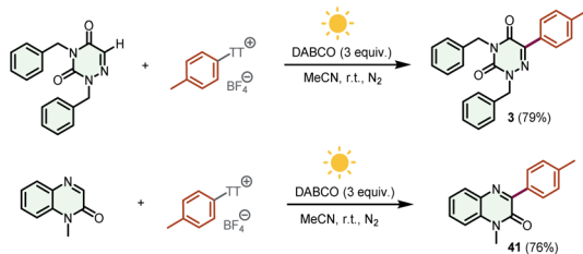
Scheme 5 Synthetic applications.
