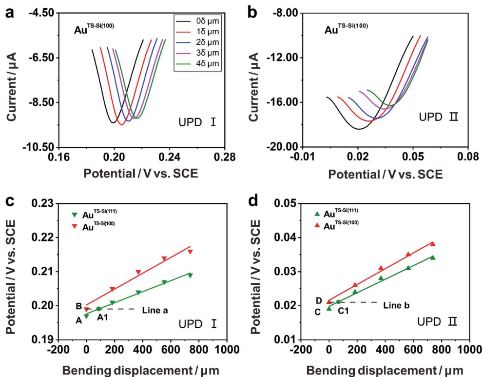
Fig. 3 Cyclic voltammograms of Cu UPD on quasi-single-crystal Au TS-Si(100) films under different strain conditions. (a) Cu UPD I on the Au TS-Si(100) film; (b) Cu UPD II on the Au TS-Si(100) film in an aqueous solution containing 1 mM CuSO 4 and 50 mM H 2 SO 4 . The scan rate of the potential was 10 mV s -1 . The inset in (a) represents the varying bending displacement of the film, which was utilized to modulate the strain of the film. Evolution of the underpotential of (c) Cu UPD I and (d) Cu UPD II, along with bending displacement of the Au film. In particular, green for the Au TS-Si(111) film, and red for the Au TS-Si(100) film. The bottom dashed lines (line a and line b) represent the contour plot of the electrochemical activity for Cu UPD I and Cu UPD II of the Au TS-Si(100) film without bending. A1 and C1 are points where line a intersects the green line and line b intersects the green line, indicating the electrochemical activities for Cu UPD I and Cu UPD II of the Au TS-Si(111) film are equal to that of an unbending Au TS-Si(100) one at such bending displacements.
