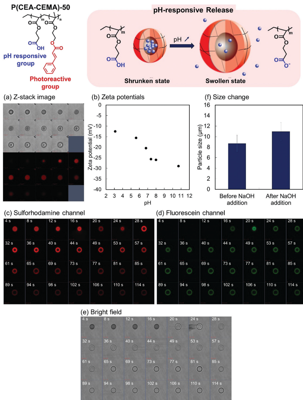
Fig. 5 (a) CLSM images (z-stack images) of P(CEA-CEMA)-50 capsule particles containing sulforhodamine B. Interval of z-stack images is 1 \mu m. Top: Bright image. Bottom: Fluorescence image. (b) Zeta potential of P(CEA-CEMA)-50 hollow particles at various pH conditions. Time-lapse CLSM images of P(CEA-CEMA)-50 capsule particles containing sulforhodamine B after addition of NaOH granules: (c) sulforhodamine B channel, (d) fluorescein channel, and (e) bright field. (f) Average particle size of polymer capsules before (left) and after (right) NaOH addition. P(CEA-CEMA): poly(2-carboxyethylacrylate-co-2-cinnamoyl ethyl methacrylate).
