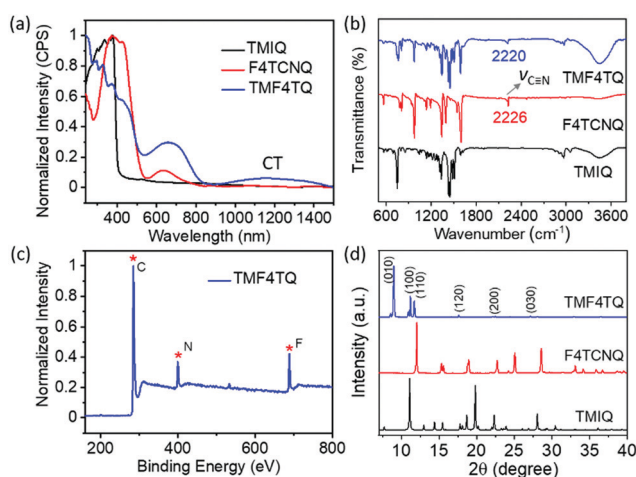
Fig. 2 (a) UV-vis-NIR absorption, (b) FTIR spectra, and (d) PXRD patterns of powders for TMIQ, \text{F}_4\text{TCNQ} , and TMF4TQ cocrystals. (c) Full scan of XPS for the cocrystal TMF4TQ.
