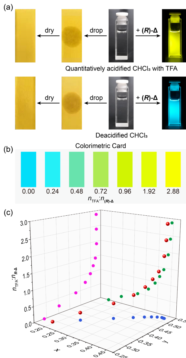
Fig. 4 Detecting traces of acids employing (R)- \Delta . (a) Fluorescence changes of solutions (right) of (R)- \Delta in CHCl 3 with and without TFA upon shining 365 nm-UV light in comparison with detecting trace acid in the same solvents using pH papers (left). (b) A colorimetric card showing the ability of (R)- \Delta to detect visually amounts of acid in solutions with different n_{\text{TFA}}:n_{(\text{R})-\Delta} ratios. (c) The fitting function based on the PL emission of (R)- \Delta upon changing the n_{\text{TFA}}:n_{(\text{R})-\Delta} ratio from 0.00 to 2.88. The concentration of (R)- \Delta is 1 \times 10^{-5} M.
