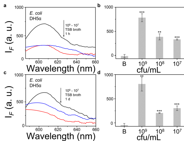
Fig. 1 TCF-Nitro based fluorescence detection (a), (c) and corresponding change in fluorescence (b), (d) with 1–100 times diluted TSB-cultured E. coli DH5 \alpha (approx. 10^9 \text{ CFU mL}^{-1} ) to determine NTR activity and probe detection limits, under 1 h and 1 d detection periods respectively. Black: 10^9 \text{ CFU mL}^{-1} group. Red: 10^8 \text{ CFU mL}^{-1} group. Blue: 10^7 \text{ CFU mL}^{-1} group. ^{**}P < 0.01 , ^{***}P < 0.001 . \lambda_{\text{ex}} = 560 \text{ nm} , \lambda_{\text{em}} = 606 \text{ nm} .
