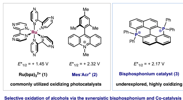
Fig. 1 Photocatalytic selective oxidation of benzylic alcohols via synergistic bisphosphonium and cobalt catalysis.
