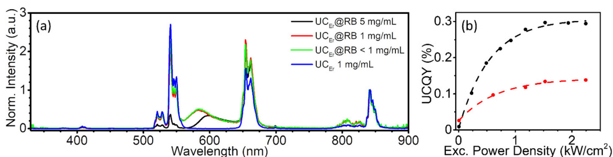
Fig. 5 (a) 841 nm-normalized corrected UC emission spectra of \text{UC}_{\text{Er}} and \text{UC}_{\text{Er}}@\text{RB} dispersions at different concentrations ( \lambda_{\text{exc}} = 980 nm; I = 2.1 W \text{cm}^{-2} ). (b) Power density dependency of absolute UCQY for \text{UC}_{\text{Er}} and \text{UC}_{\text{Er}}@\text{RB} dispersions in DMF (5 mg \text{mL}^{-1} ).
