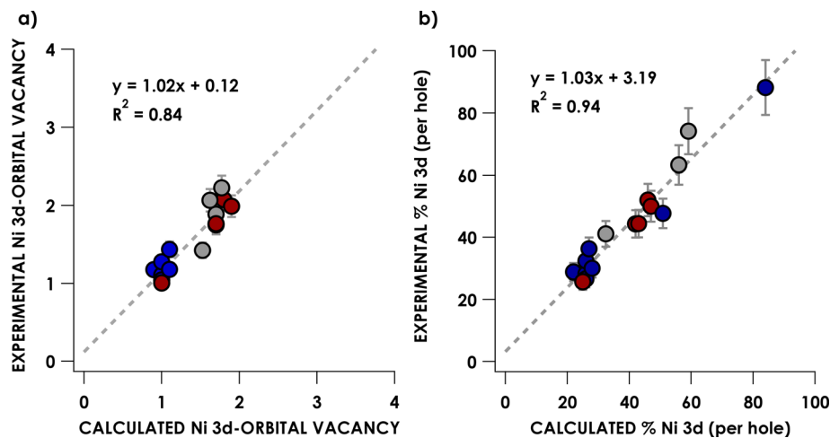
Fig. 6 Correlation between (a) experimental 3d vacancy and (b) experimental % Ni 3d character per acceptor hole with DFT-calculated values for formally \text{Ni}^{\text{III}} (blue), \text{Ni}^{\text{III}} (grey), and \text{Ni}^{\text{IV}} (red) species. Errors in slope and y-intercept, respectively, are (a) \pm 0.06 , \pm 0.03 ; (b) \pm 0.07 , \pm 0.09 .
